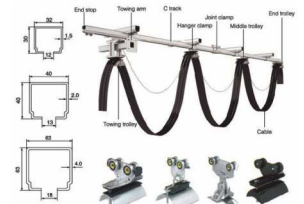
Festooned System
